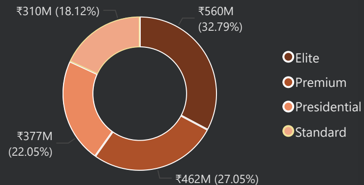
Total Revenue by Room Class
